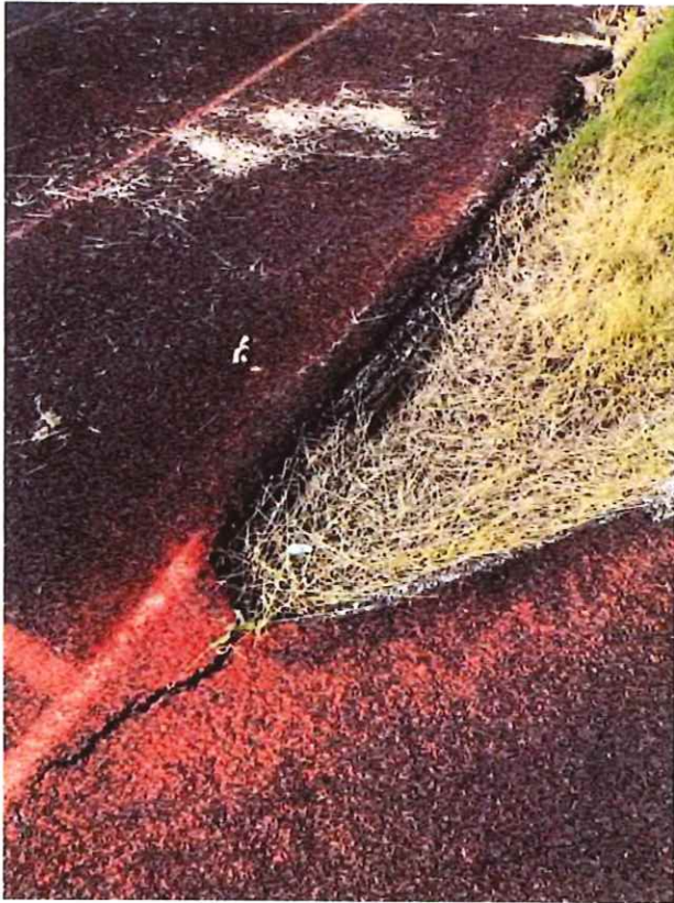
Track Layers at Starting Box
